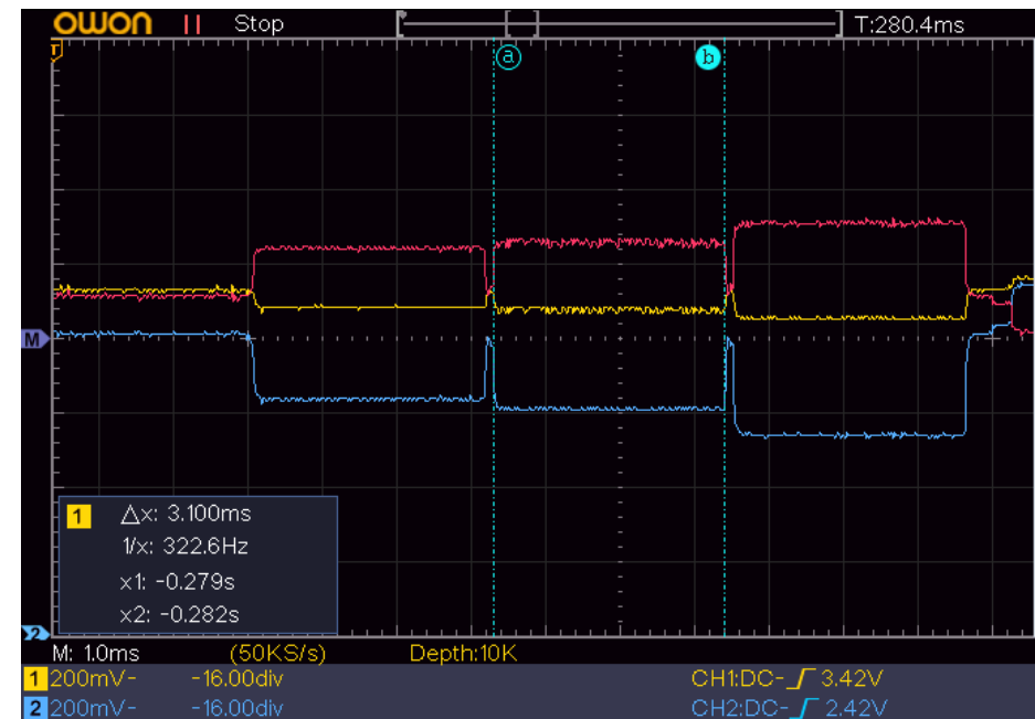
DUT NanoB#25, 125K PHY Advertising Time ~3.1ms for Each Adv. Channel
