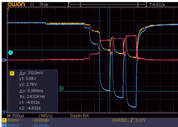
Channel 37 Peak Current ~31.2mA
