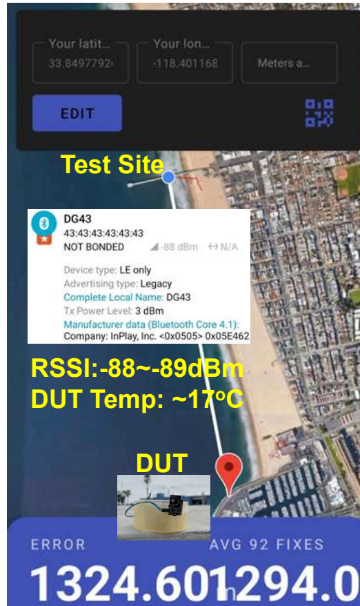
Range Test Result LOS Range ~ 1.32km
