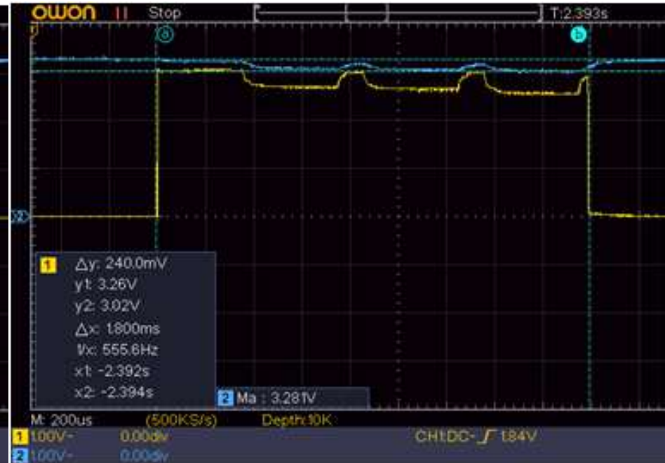
Example SW0 Waveform SW0 ON Time ~1.8ms
