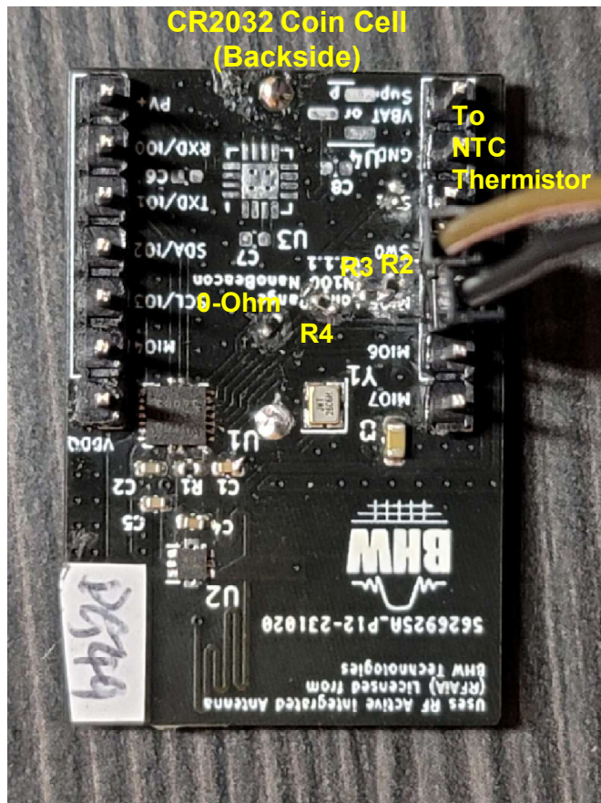
NanoBeacon with Double Voltage Divider and NTC Thermistor
