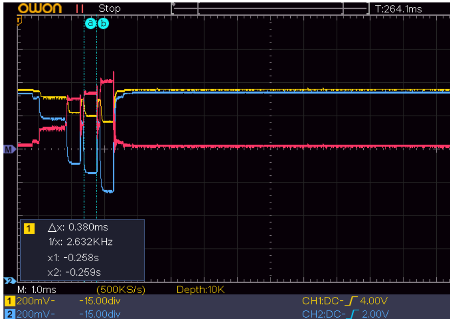
DUT NanoB#66, 1M PHY Advertising Time ~0.38ms for Each Adv. Channel
