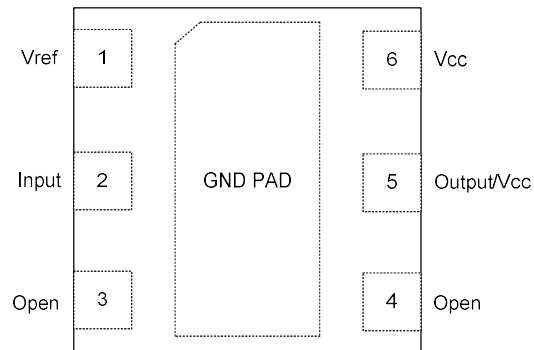
(Top "See-Through" View)
